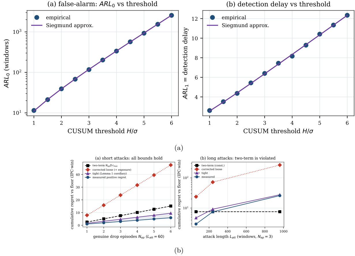
Figure 18: Theory. (a) ARL matches Siegmund; (b) the safety-floor bound envelopes measured regret.
