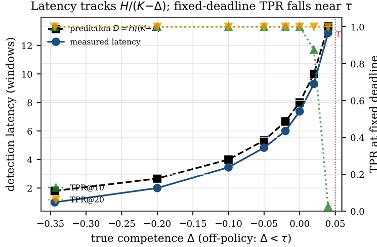
Figure 16: Detection latency vs. competence gap (positive form of Figure 15(d)). Every gap eventually gates (full-duty drift 3.8\text{--}28\sigma_\Delta ; 1.9\text{--}14\sigma_\Delta background), but the detection latency rises from 1 to 13 windows toward the \tau boundary, tracking the deterministic-drift limit H/(K - \Delta_W) , so the fixed-deadline TPR falls (TPR by 10 windows drops to 0.03 at \Delta_W=0.04 , recovering to 1.0 by 20).
