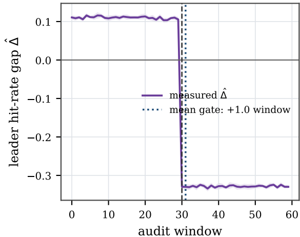
(b) Competence, not inputs, exposes the reversal
