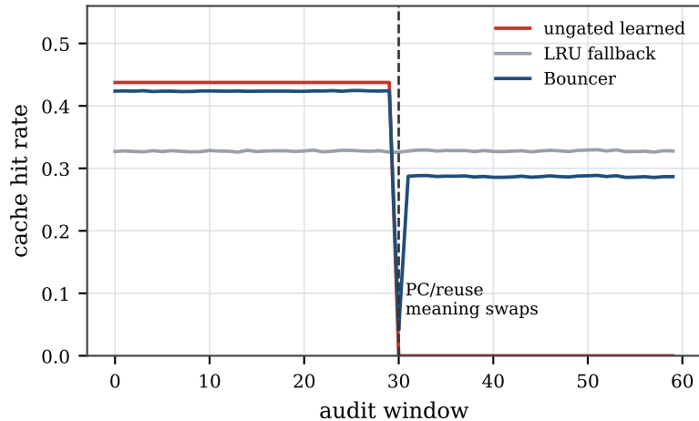
(a) Learned gain reverses under concept shift
