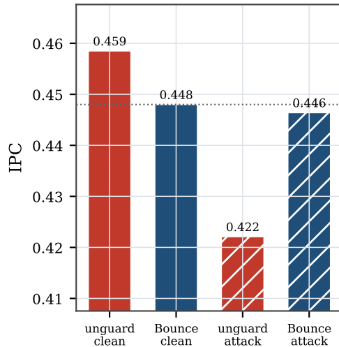
SPEC 619.lbm_s (clean tax 2\%)
