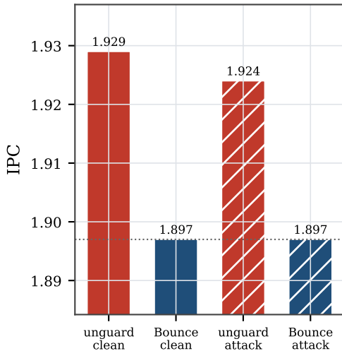
SPEC 600.perlbench_s (clean tax 2\%)
