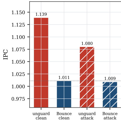
SPEC 654.roms_s (clean tax 11\%)
