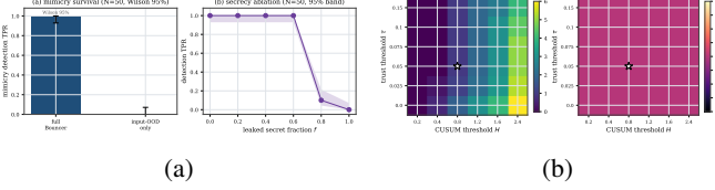
Fig. 10: Robustness. (a) headline results over 50 seeds with Wilson 95% intervals; (b) sensitivity of detection latency and clean false-alarm rate to (\tau, H) —the operating point (\star) sits on a broad plateau.
