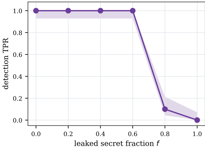
(b) secrecy ablation (N=50, 95% band)
