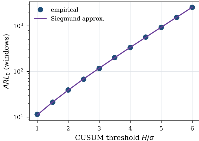
(a) false-alarm: ARL_0 vs threshold
