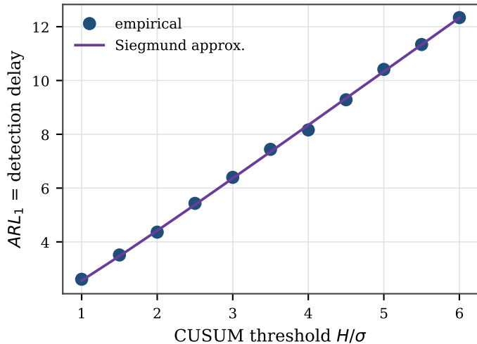
(b) detection delay vs threshold
