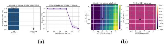
Fig. 10: Robustness. (a) headline results over 50 seeds with Wilson 95% intervals; (b) sensitivity of detection latency and clean false-alarm rate to (\tau, H) —the operating point (★) sits on a broad plateau.
