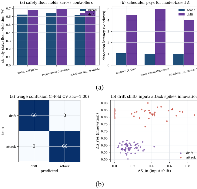
Fig. 8: P3. (a) the floor holds across controller classes; (b) attack-vs-drift triage (acc 1.0).
