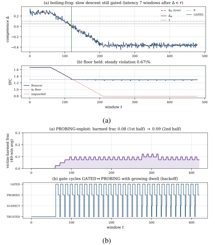
Fig. 13: Adaptive timing adversaries. (a) boiling-frog is still gated (a CUSUM integrates level, not slope); (b) the PROBING-exploit attacker is bounded to 8.6% harmed windows by measured re-trust + dwell backoff.
