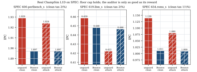
Fig. 16: Bouncer as a real ChampSim L1D prefetcher across a SPEC suite. On every trace Bouncer ends at the prefetch-off floor (the cap), bounding the corruption attack’s worst case (lbn: 7.9% unguarded loss cannot reach the gated victim). The per-set cache-hit reward proxy sets the clean tax (1.7–11%); roms shows the failure mode—a genuinely-helpful prefetcher under-credited and over-gated. Swapping to the controller’s own reward does not fix this (only 11.2% \rightarrow 9.7%); a prefetcher’s benefit is not set-local, so set-dueling needs a longer epoch or a set-local signal (replacement is the set-local case—though a real cache’s stateful reward is a further boundary; see Section XI-J).
