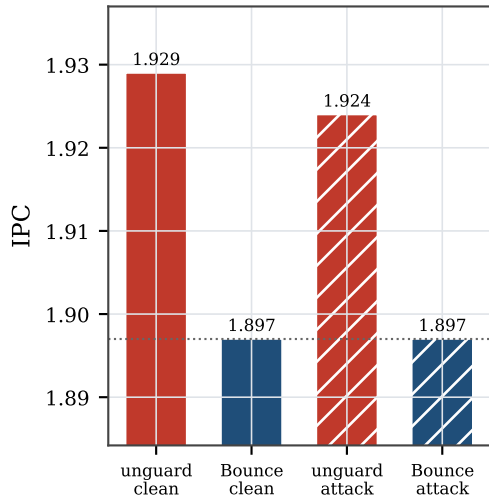
SPEC 600.perlbench_s (clean tax 2%)
