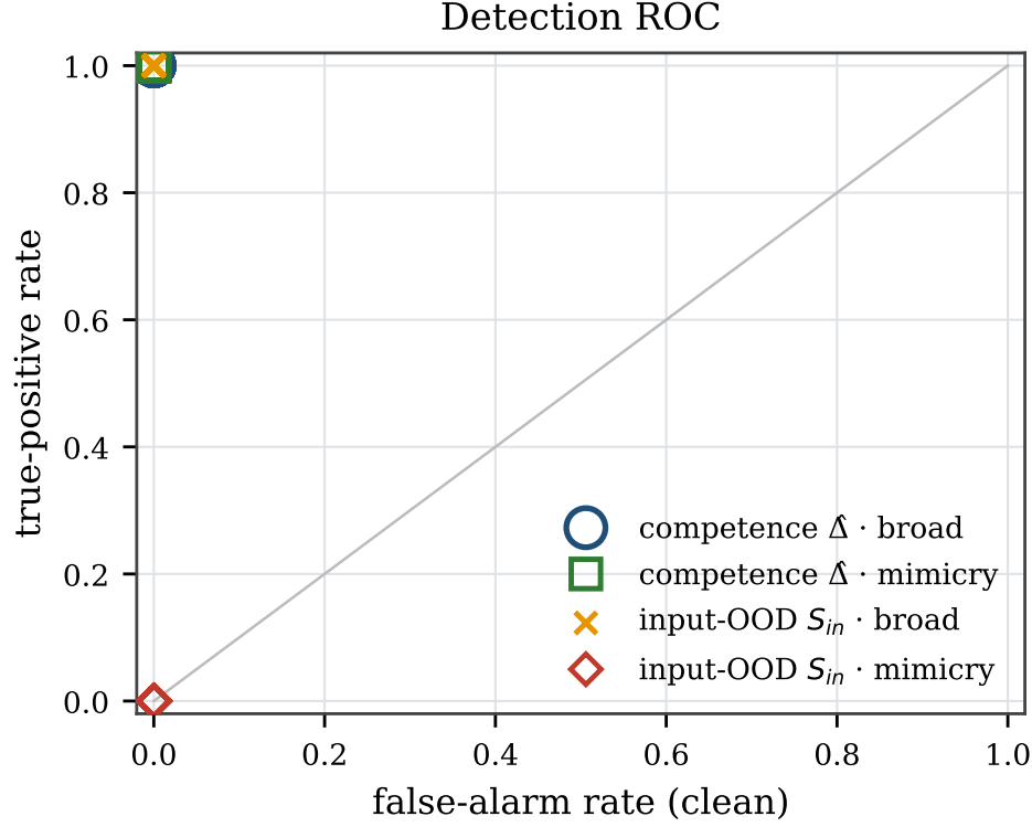
Figure 8: P2 threshold-sweep operating points. Every tested threshold collapses to the marked point: the competence detector catches broad and mimicry attacks; S_{in} catches only the broad attack. Coincident markers at (0, 1) are nested.
