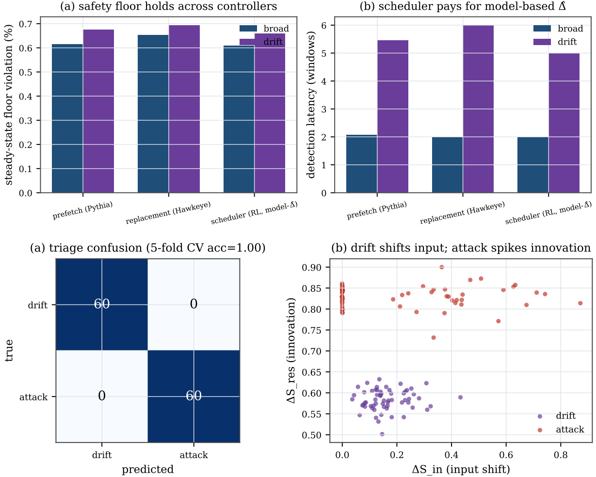
Figure 10: P3 synthetic abstractions. Top: the floor holds across three harness instantiations. Bottom: attack and drift are separable within the constructed episode family (five-fold accuracy 1.0).
