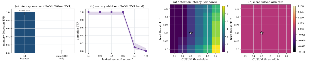
Figure 12: Robustness. Left: headline results over 50 seeds with Wilson 95% intervals. Right: sensitivity of detection latency and clean false-alarm rate to (\tau, H) —the operating point ( \star ) sits on a broad plateau.
