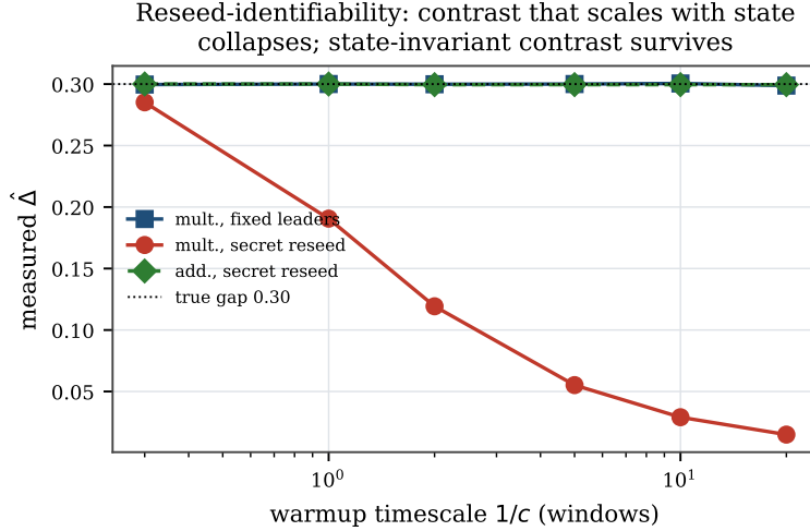
Figure 14: Synthetic warm-up model. With a multiplicative warm-up contrast, secret reseed returns almost every sampled slice to the cold state and attenuates \hat{\Delta} ; fixed leaders recover the 0.30 gap. An equally stateful additive warm-up with state-invariant contrast remains identifiable. This isolates a mechanism; it is not evidence about real predictors.
