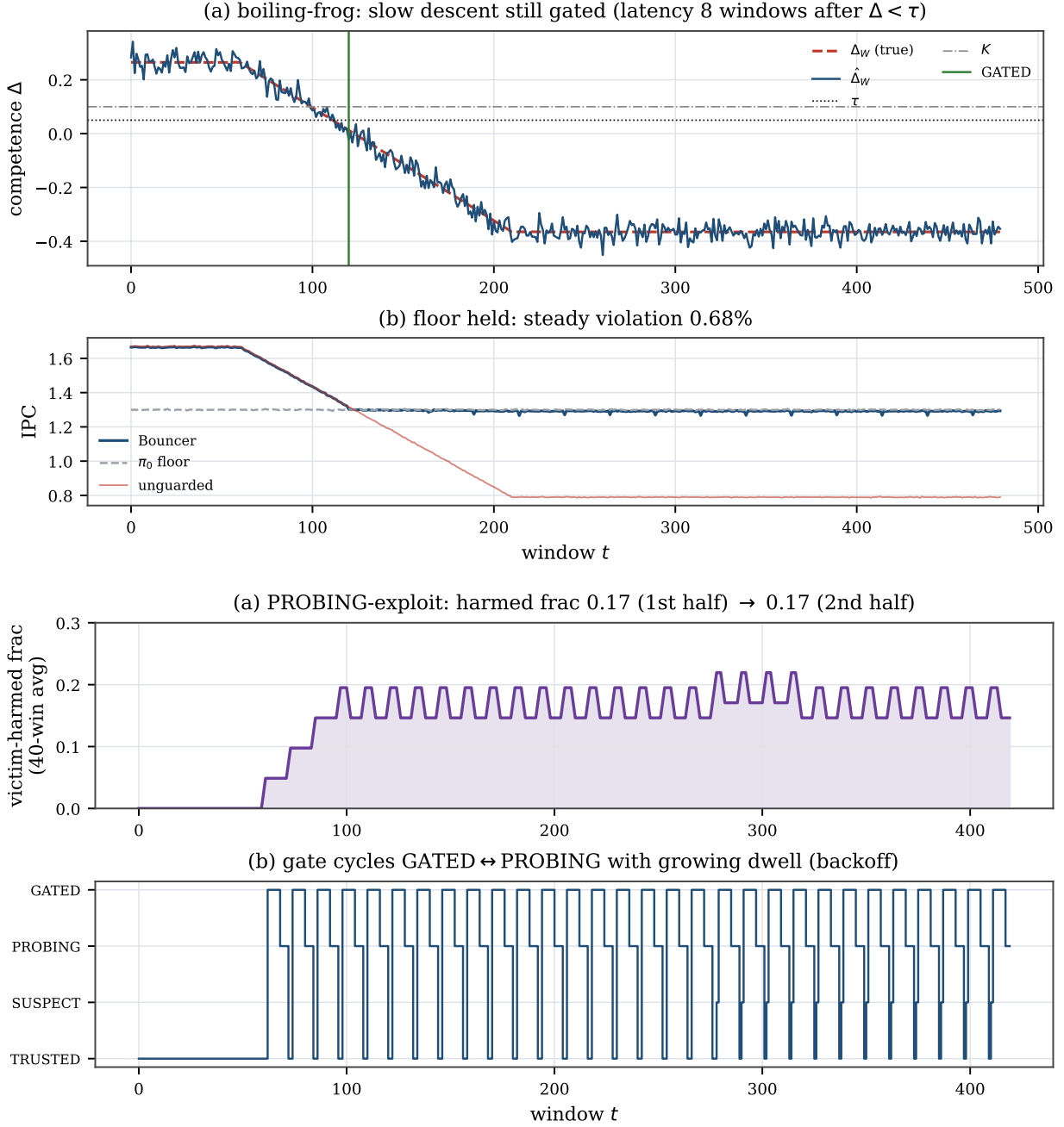
Figure 17: Adaptive timing adversaries. Top: boiling-frog is still gated (a CUSUM integrates level, not slope). Bottom: the PROBING-exploit attacker is bounded to a small harmed-window fraction (16.9%) by measured re-trust and dwell backoff.
