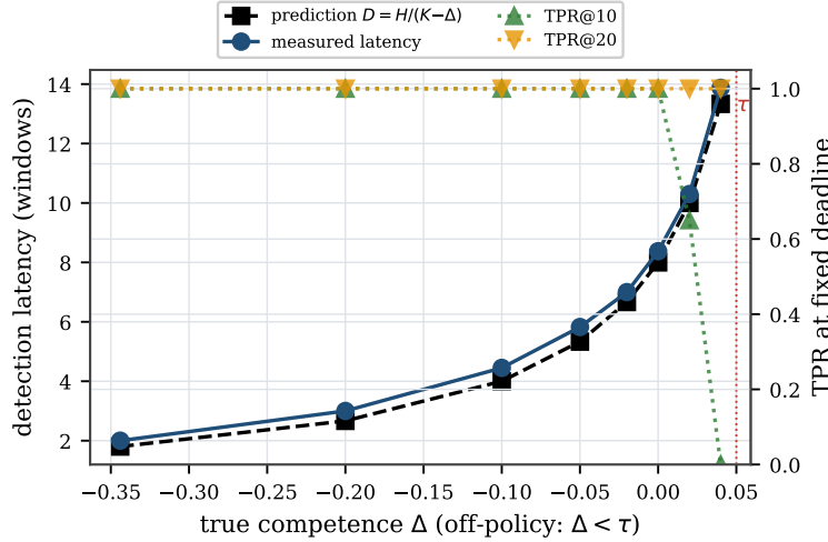
Figure 16: Detection latency vs. competence gap (positive form of Figure 15(d)). Every tested gap gates within 40 windows (full-duty drift 3.8\text{--}28\sigma_\Delta ; 1.9\text{--}14\sigma_\Delta background), but detection latency rises from 2 to 13.9 windows toward the \tau boundary, tracking the deterministic-drift limit H/(K - \Delta_W) , so the fixed-deadline TPR falls (TPR by 10 windows drops to 0 at \Delta_W=0.04 , recovering to 1.0 by 20).
