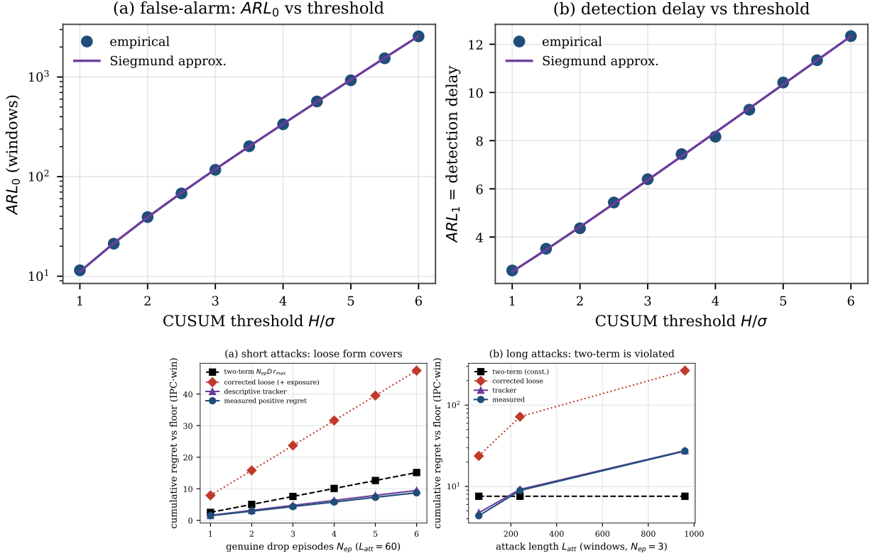
Figure 18: Theory. Top: ARL matches Siegmund. Bottom: measured regret versus the two-term expression, loose three-term plug-in, and descriptive tracker.
