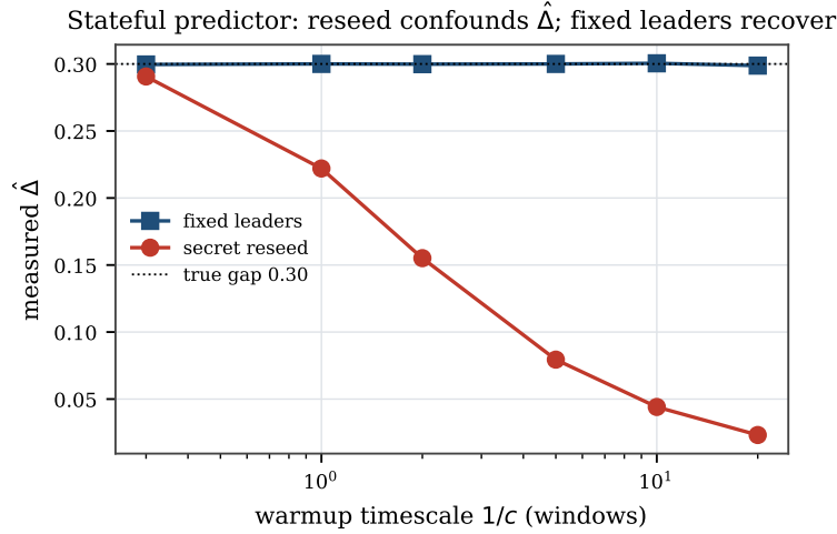
Figure 12: Stateful predictor (accuracy warms up over consecutive windows on a policy). As the warmup timescale 1/c lengthens, the secret reseed keeps both pools cold so \hat{\Delta} attenuates toward noise, while fixed leaders recover the true 0.30 gap. Generalizes the ChampSim replacement reseed-confound beyond the cache.
