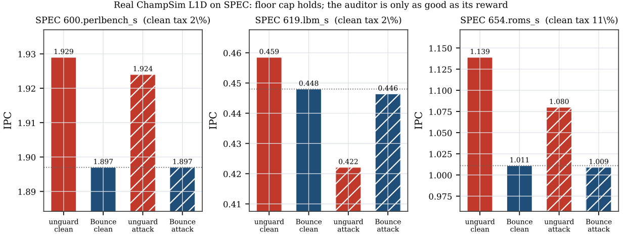
Figure 18: Bouncer as a real ChampSim L1D prefetcher across a SPEC suite. On every trace Bouncer ends at the prefetch-off floor (the cap), bounding the corruption attack’s worst case (lbm: 7.9% unguarded loss cannot reach the gated victim). The per-set cache-hit reward proxy sets the clean tax (1.7–11%): roms shows the failure mode—a genuinely-helpful prefetcher under-credited and over-gated. Swapping to the controller’s own reward does not fix this (only 11.2% \rightarrow 9.7%); a prefetcher’s benefit is not set-local, so set-dueling needs a longer epoch or a set-local signal (replacement is the set-local case—though a real cache’s stateful reward is a further boundary; see Section 11.10).
