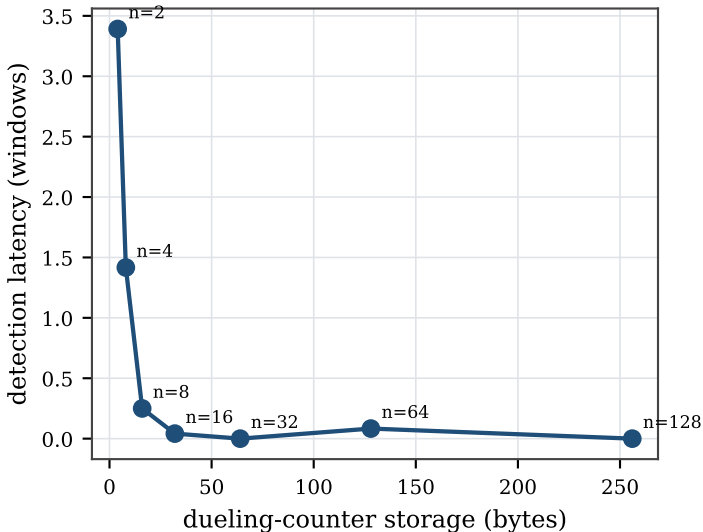
Overhead \rightarrow latency Pareto frontier
