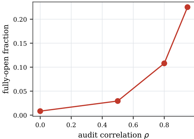
(B) correlated (stateful) audit inflates D (reseed-id. boundary)
