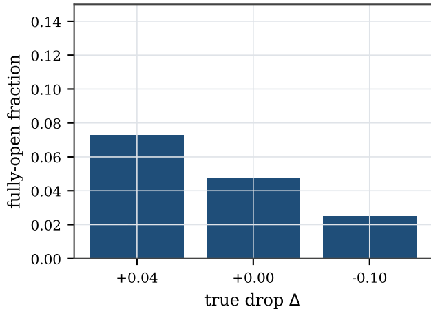
(A) reseeded i.i.d. audit: D small (detection+SUSPECT)
