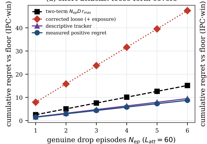
(a) short attacks: loose form covers
