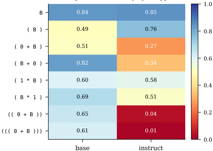
multiplication accuracy by wrapper
