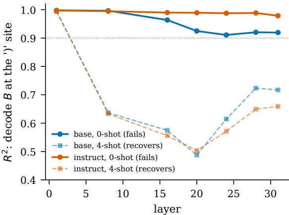
Operand decodable at every layer (0-shot)
