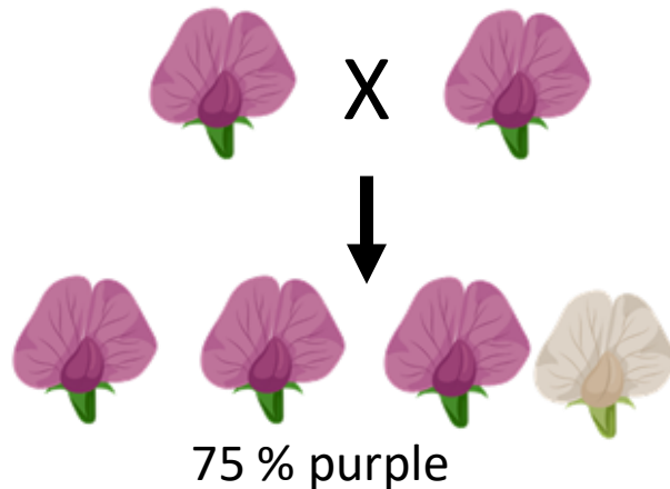
Result D
