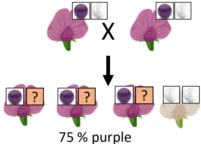
Result D
