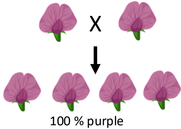
Result C
