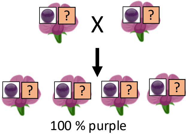
Result C
