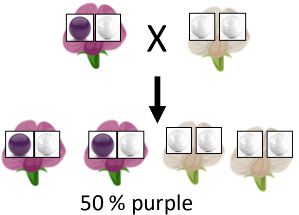
Result B
