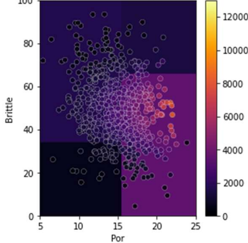
Training Data and Boosting with 1 Trees
