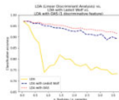
Normal, Ledoit-Wolf and OAS Linear Discriminant Analysis for classification
