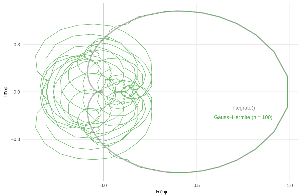
Lognormal CF at \sigma = 1
