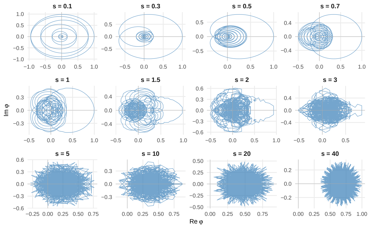
Lognormal characteristic function in the complex plane
