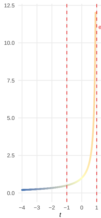
Lognormal characteristic function in the complex plane
