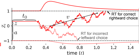
B. Choices and Reaction Times for Two Trials
