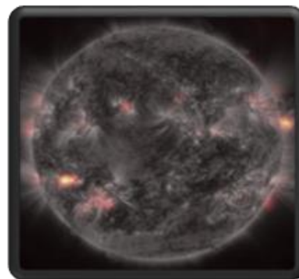
Flare Localization
