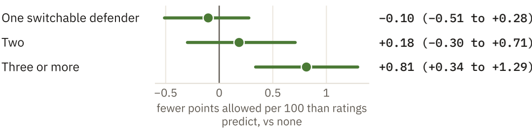
FIGURE 10 Lineups with more switchable defenders allow fewer points than their ratings predict
