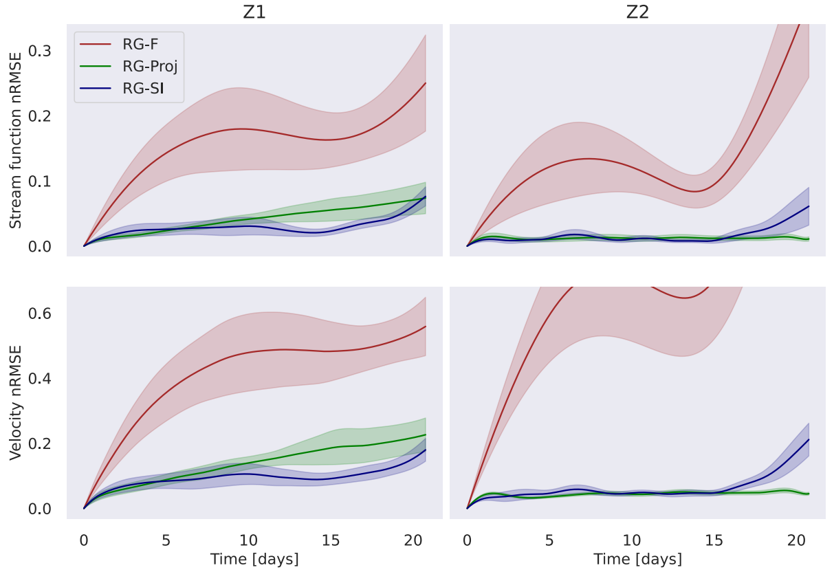
Figure C1. nRMSE on surface stream function (top row) and velocities (bottom row), averaged over 12 20-days periods, each separated by 20 days, on Z1 (left) and Z2 (right). Standard RG-SI model is identified by the solid blue line, RG-SI with coefficient obtained through the projection of \psi_2 (from the reference three-layer QG model) onto the reduced order space is shown by the green line and RG-F by the brown one. Y-axis is shared by both panels.
