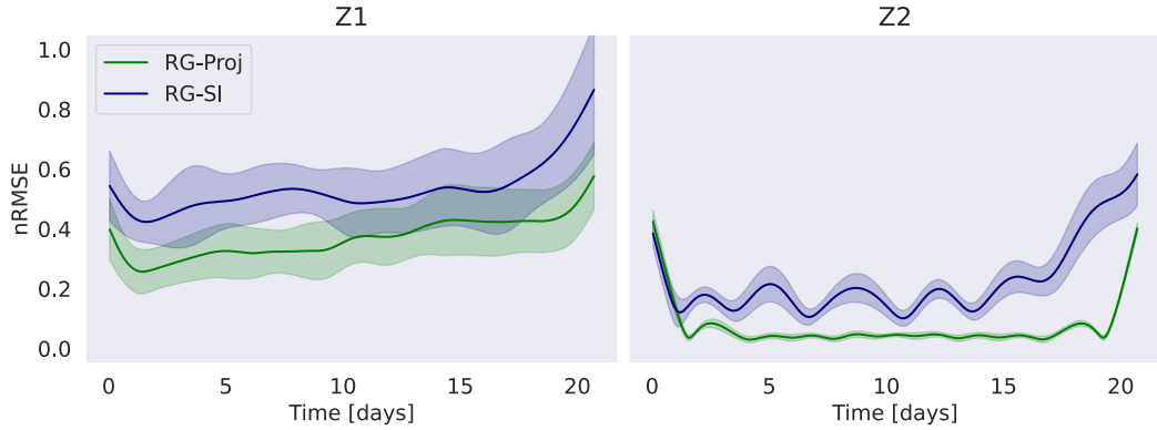
Figure C1. nRMSE on surface stream function (top row) and velocities (bottom row), averaged over 12 20-days periods, each separated by 20 days, on Z1 (left) and Z2 (right). Standard RG-SI model is identified by the solid blue line, RG-SI with coefficient obtained through the projection of \psi_2 (from the reference three-layer QG model) onto the reduced order space is shown by the green line and RG-F by the brown one. Y-axis is shared by both panels.
