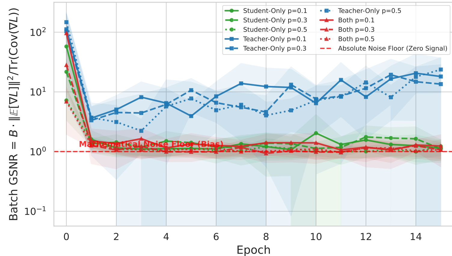
Ghost Batch GSNR Trajectory During Distillation
