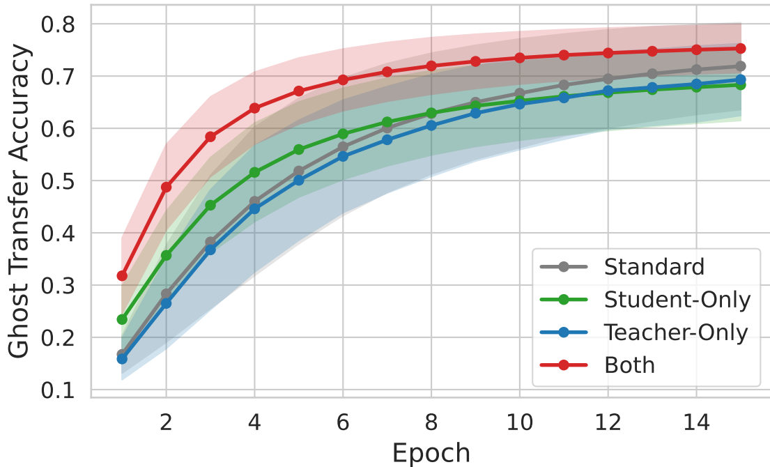
Accuracy Trajectory (L1 Centering)
