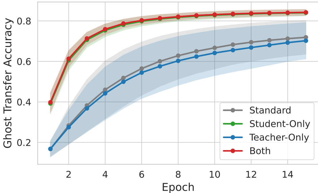
Accuracy Trajectory (L3 Centering)
