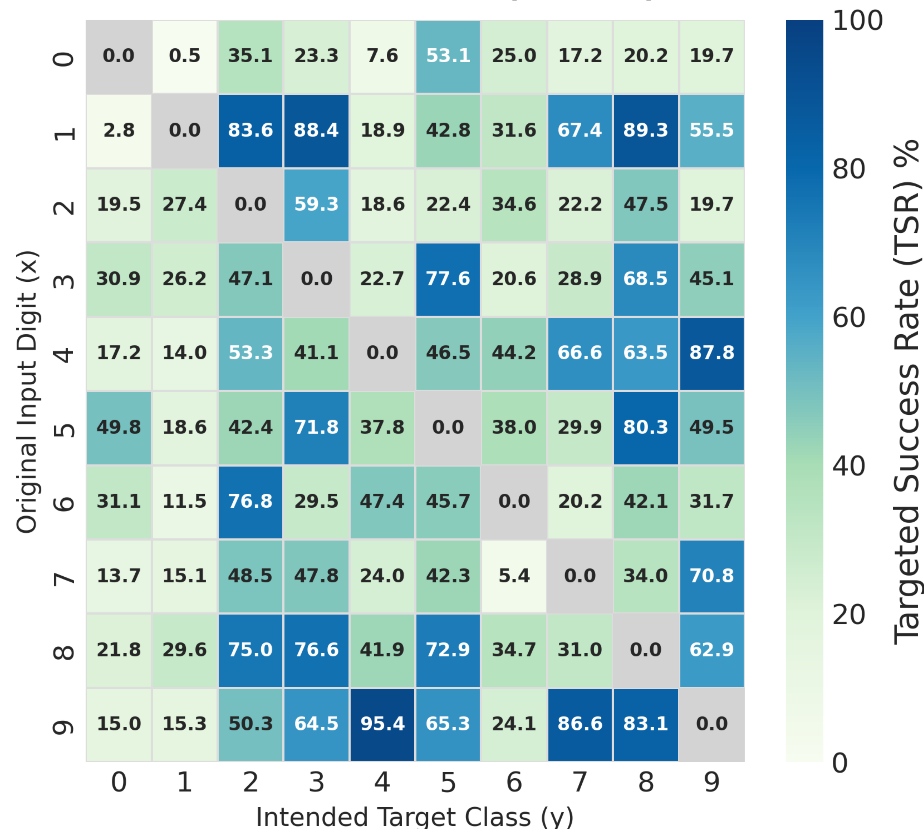
Teacher -> Teacher (Control)
