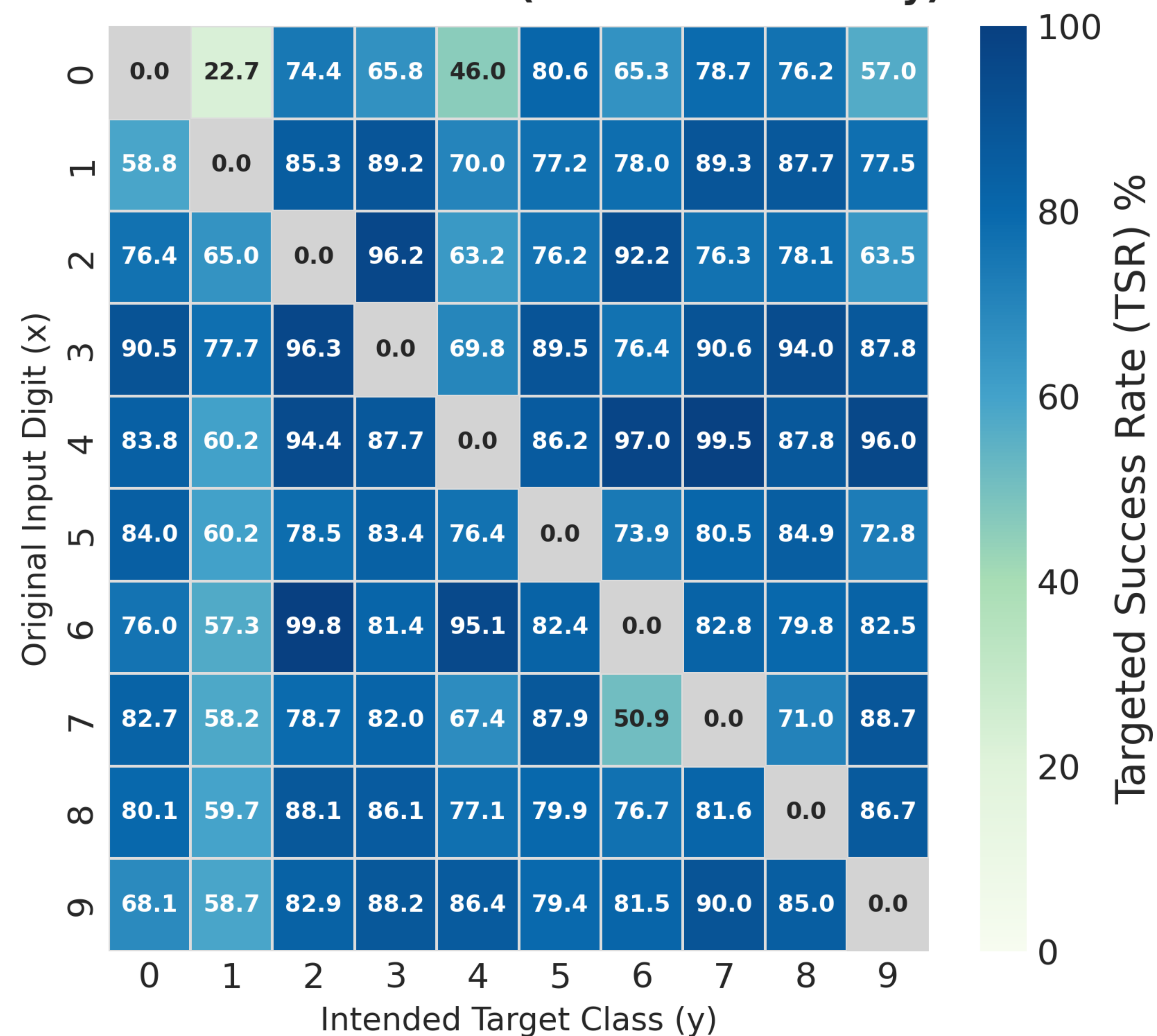
Student -> Student (Distill Consistency)
