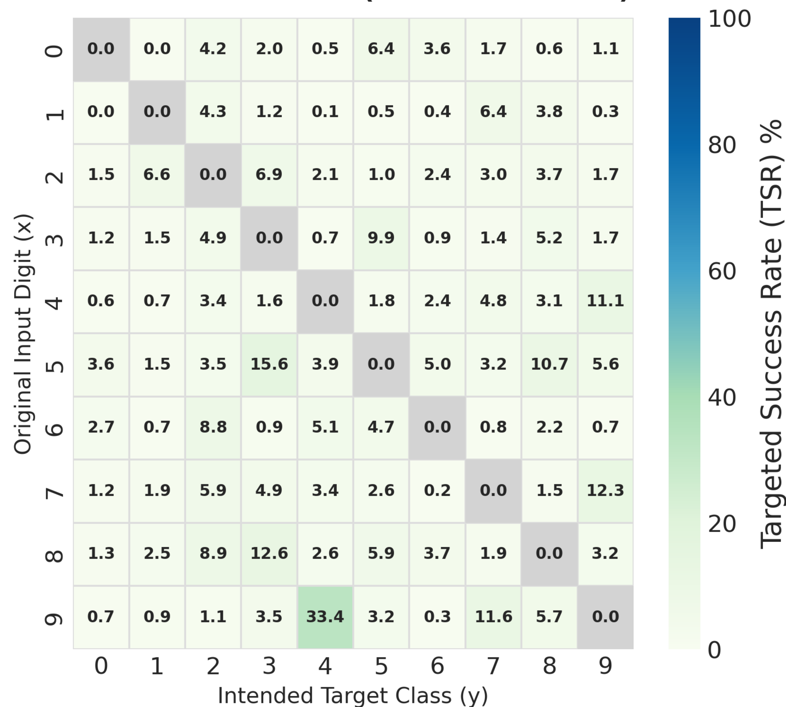
Student -> Teacher (Reverse Transfer)
