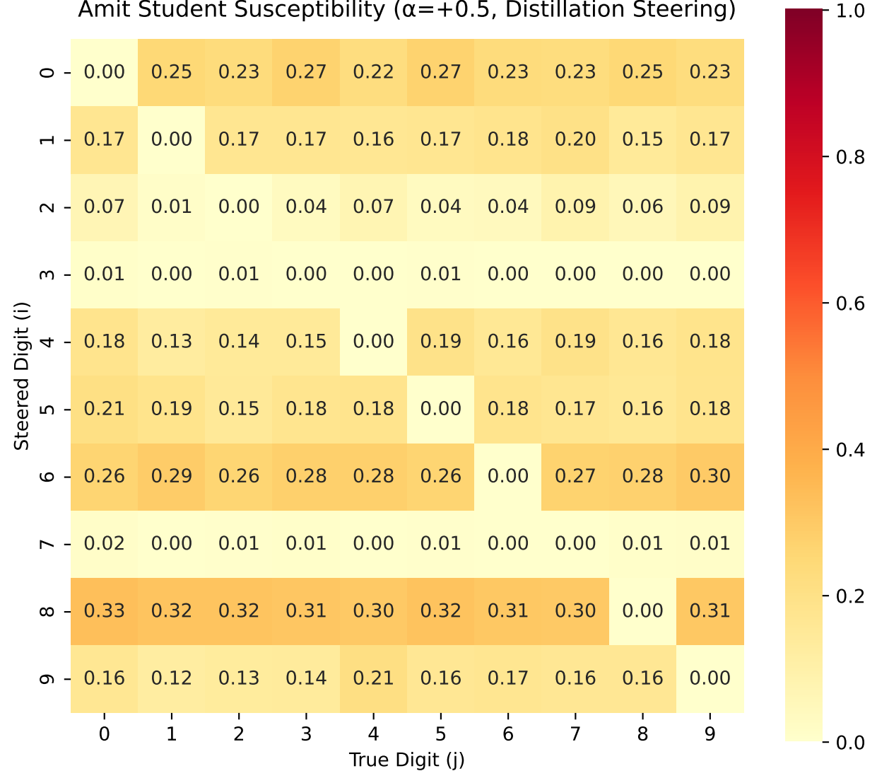
Amit Student Susceptibility ( \alpha=+0.5 , Distillation Steering)
