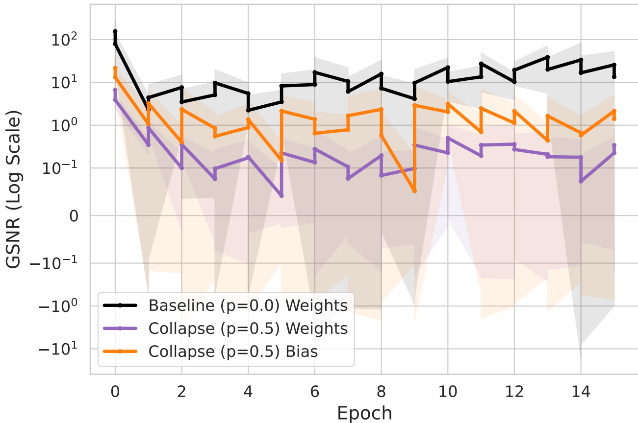
GSNR Evolution Across Distillation
