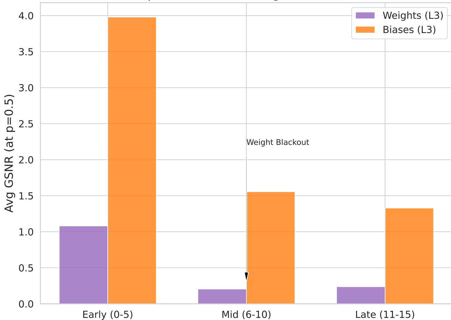
The Temporal Blackout: Weight vs Bias Survival
