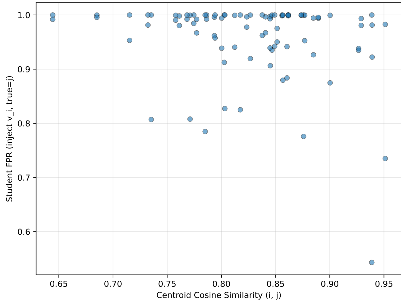
Does Geometry Predict Vulnerability?
