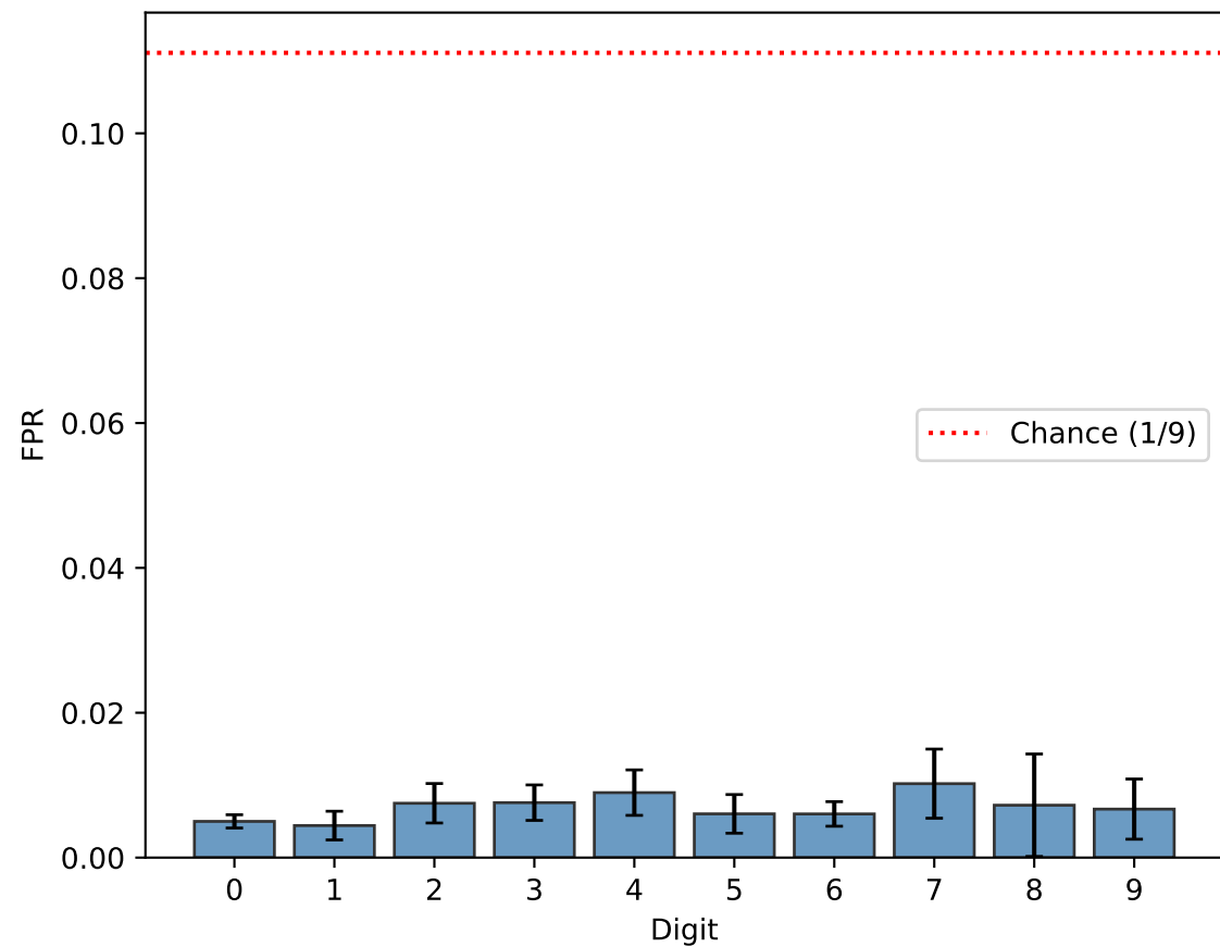
Teacher: Random Vector FPR (Acc=0.937±0.004)
