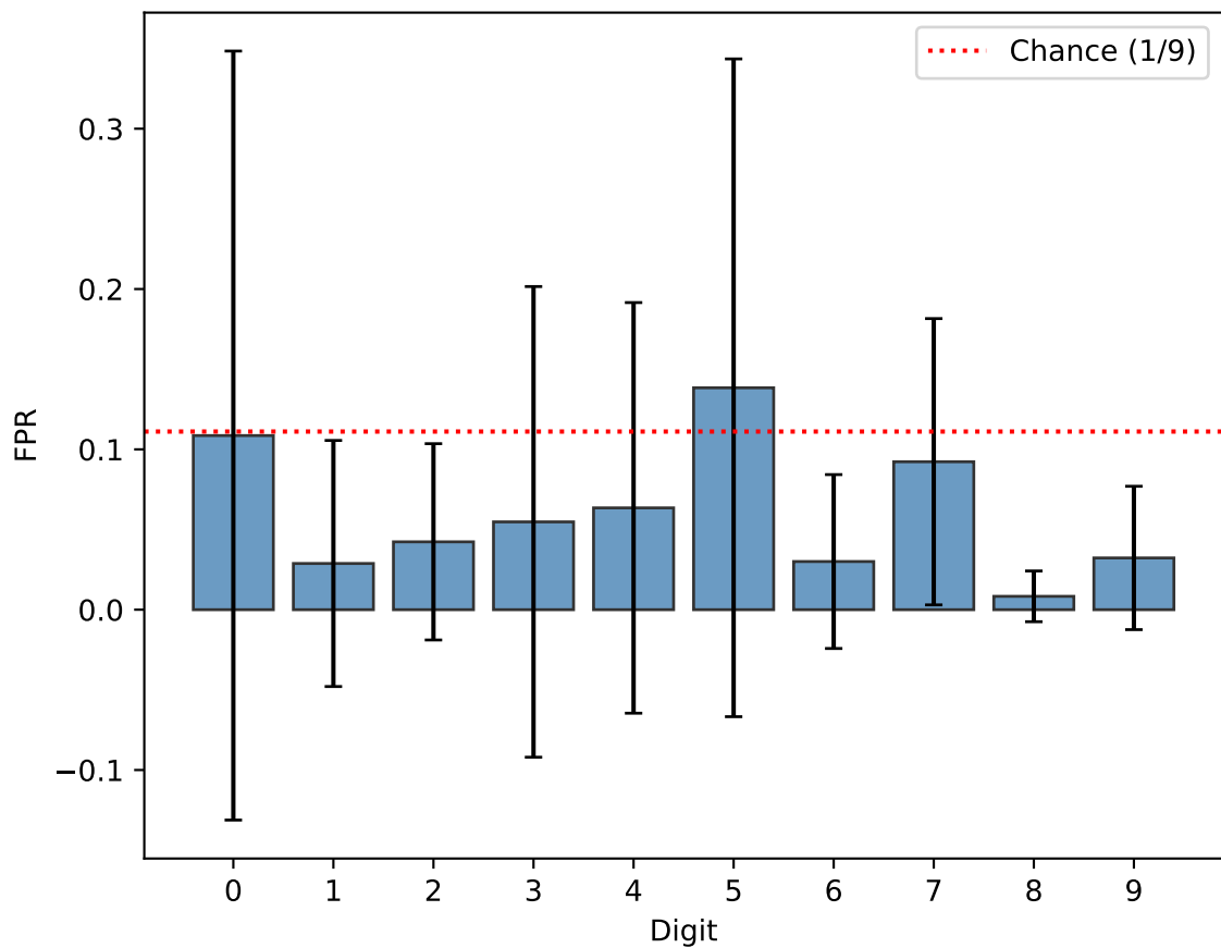
Student: Random Vector FPR (Acc=0.460±0.138)
