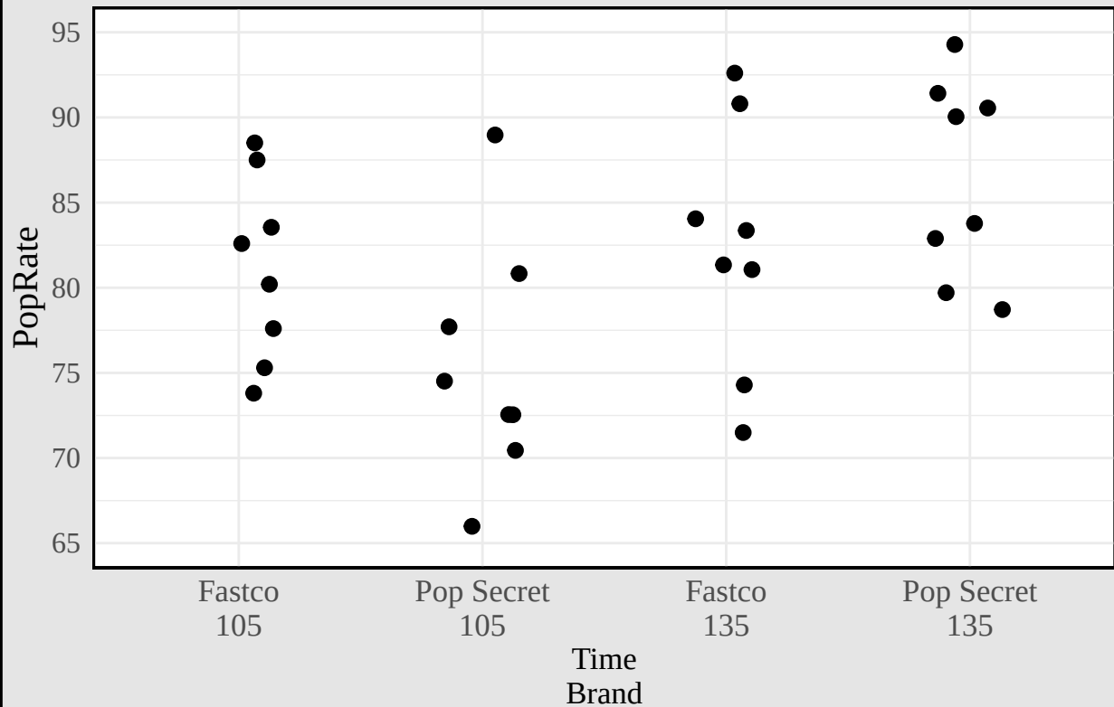
Individual Value Plot of PopRate
