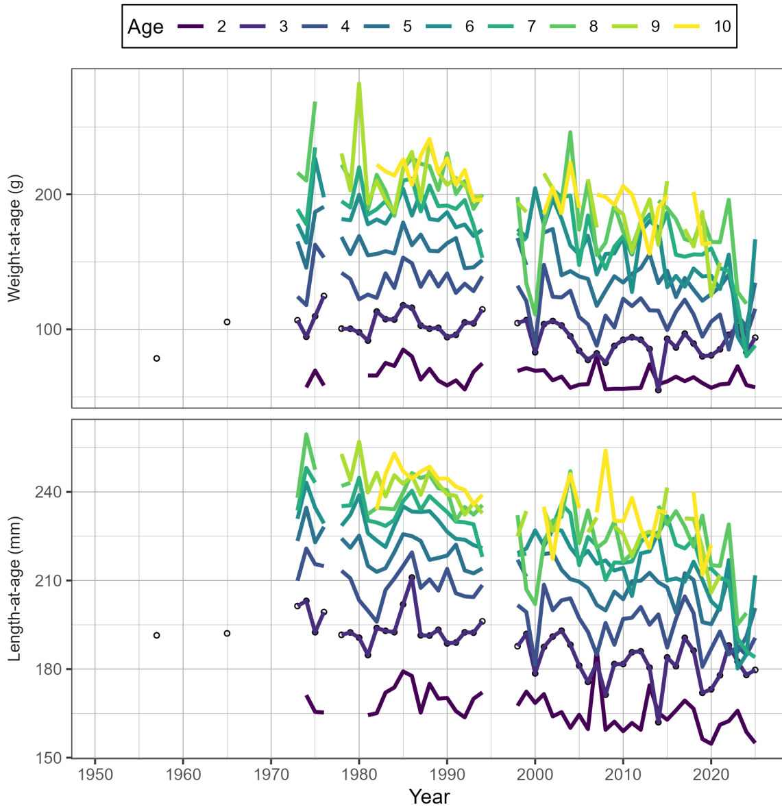
Figure 6. Time series of weight-at-age in grams (g) and length-at-age in millimetres (mm) for Pacific Herring from 1951 to 2025 in the Area 2 West minor stock assessment region (SAR). Age-3 fish are indicated by circles. Biological summaries only include samples collected using seine nets (commercial and test) due to size-selectivity of other gear types such as gillnet. The age-10 class is a ‘plus group’ which includes fish ages 10 and older.
