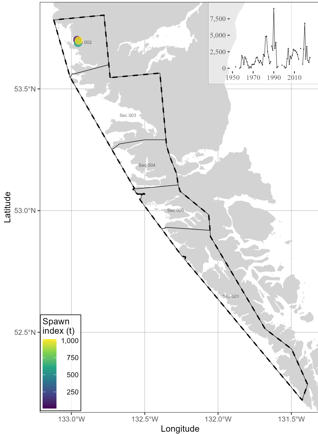
Figure 7. Pacific Herring spawn survey locations, and spawn index in metric tonnes (t) in 2025 in the Area 2 West minor stock assessment region (SAR; thick dashed lines), and associated Sections (Sec; thin solid lines). The ‘spawn index’ is not scaled by the spawn survey scaling parameter, q . Missing spawn index values indicate incomplete surveys (grey circles). Inset tracks the total spawn index. Units: kilometres (km).
