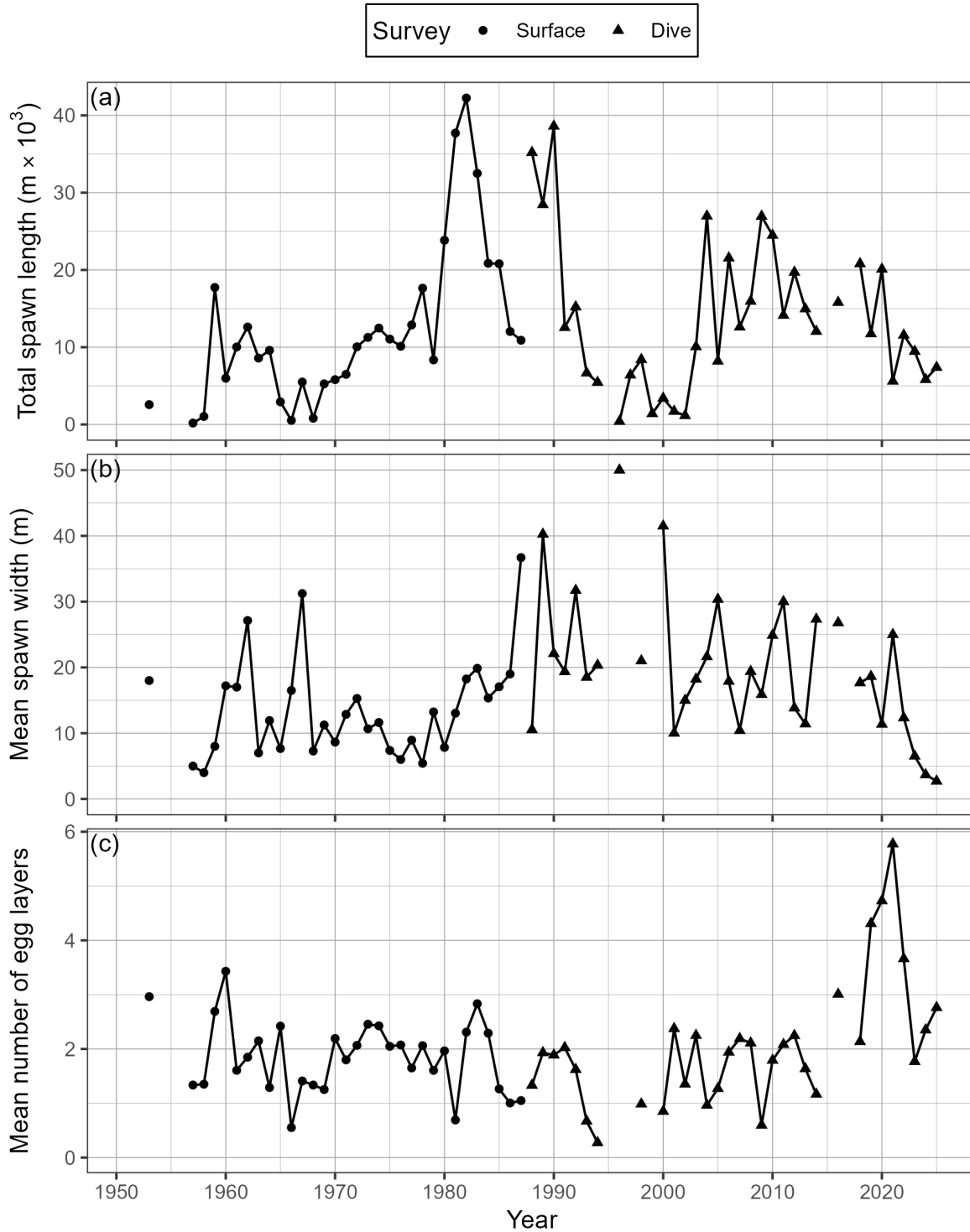
Figure 12. Time series of total spawn length in thousands of metres ( m \times 10^3 ; panel a), mean spawn width in metres (b), and mean number of egg layers (c) for Pacific Herring from 1951 to 2025 in the Area 2 West minor stock assessment region (SAR). The spawn index has two distinct periods defined by the dominant coastwide survey method: surface surveys (1951 to 1987), and dive surveys (1988 to 2025).
