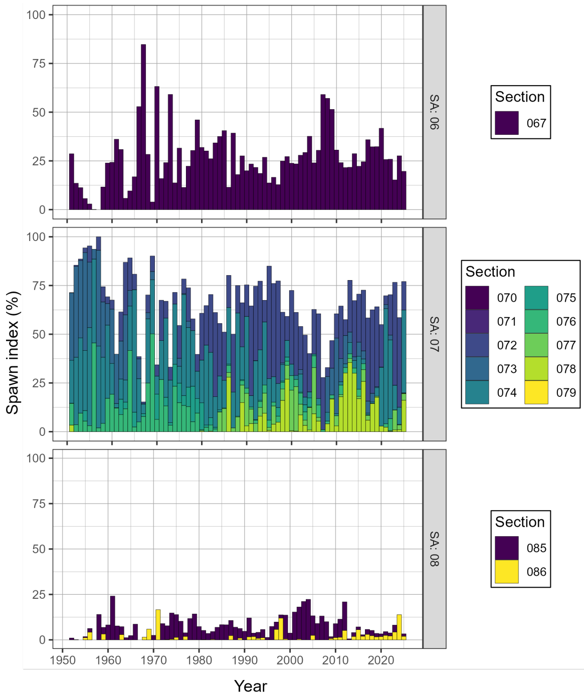
Figure 29. Time series of percent of spawn index by Statistical Area (SA) and Section for Pacific Herring from 1951 to 2025 in the Central Coast major stock assessment region (SAR). The spawn index has two distinct periods defined by the dominant coastwide survey method: surface surveys (1951 to 1987), and dive surveys (1988 to 2025). The ‘spawn index’ is not scaled by the spawn survey scaling parameter, q . Legend: ‘06&07’ is Statistical Areas 06 and 07; and ‘08’ is Statistical Area 08.
