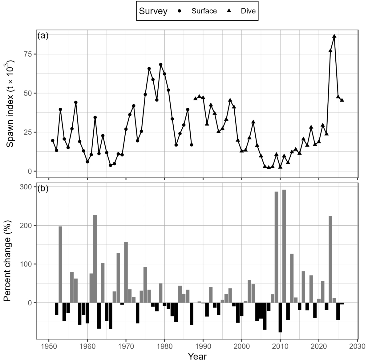
Figure 24. Time series of spawn index in thousands of metric tonnes ( t \times 10^3 ) for Pacific Herring from 1951 to 2026 in the West Coast of Vancouver Island major stock assessment region (SAR; panel a), and percent change (b). Percent change is \delta_t = \frac{\alpha_t - \alpha_{t-1}}{\alpha_{t-1}} where \alpha_t is the spawn index in year t . The spawn index has two distinct periods defined by the dominant coastwide survey method: surface surveys (1951 to 1987), and dive surveys (1988 to 2026). The ‘spawn index’ is not scaled by the spawn survey scaling parameter, q . Note that spawn surveys in the dive survey period (1988 to 2026) are a combination of surface and dive surveys (Figures 21 and 22).
