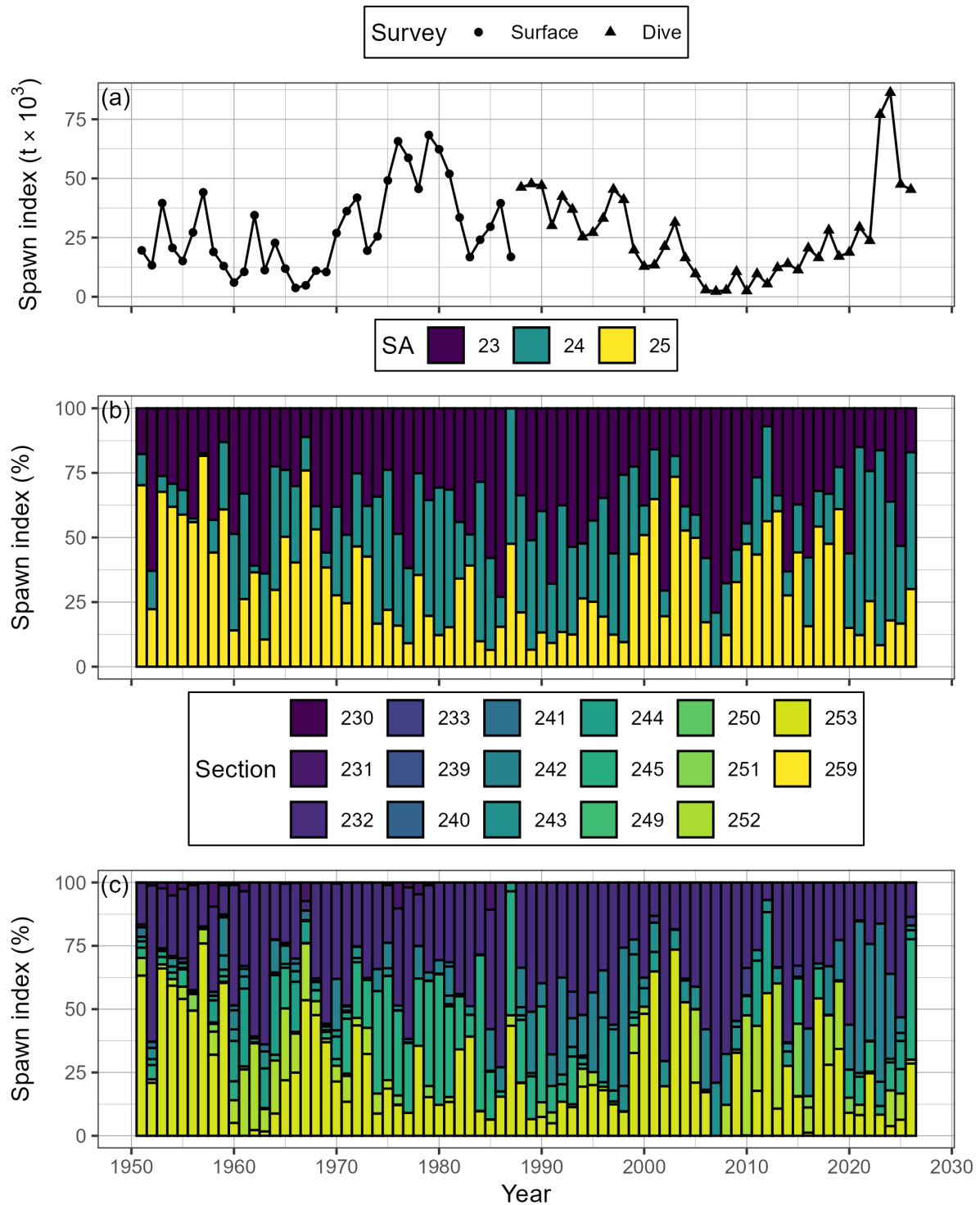
Figure 25. Time series of spawn index in thousands of metric tonnes ( t \times 10^3 ) for Pacific Herring from 1951 to 2026 in the West Coast of Vancouver Island major stock assessment region (SAR; panel a), as well as percent contributed by Statistical Area (SA), and Section (b, & c, respectively). See Figure 24 for information.
