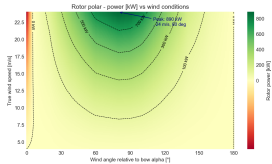
Rotor polar gain diagram.
