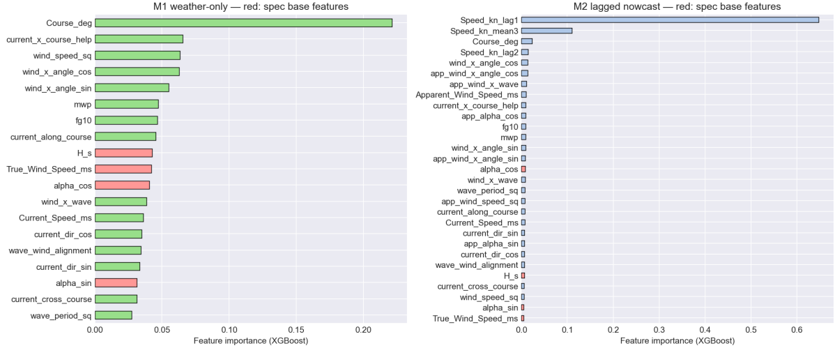
Figure 3: Feature importances for weather-only and lagged nowcast XGBoost models.
