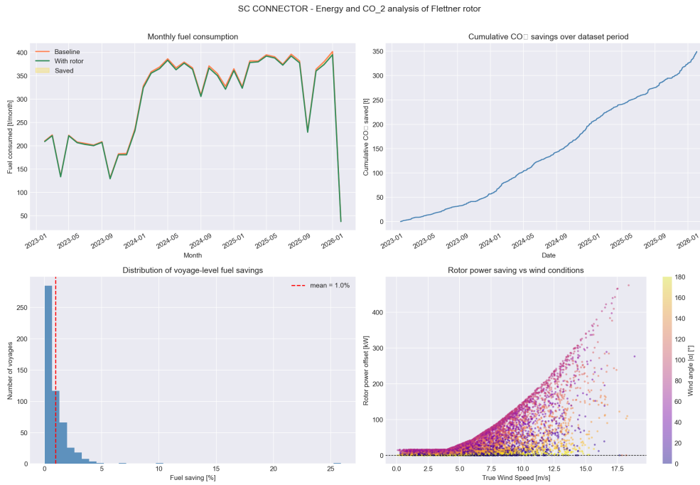
Figure 6: Fuel and CO 2 impact estimated from the rotor energy model.
