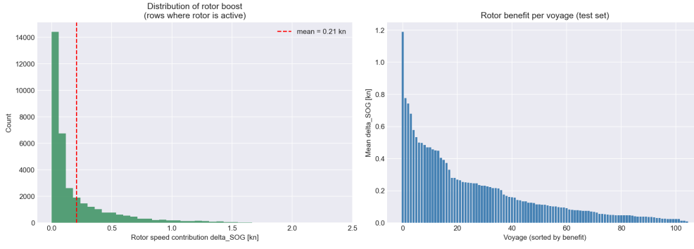
Figure 4: Rotor scenario distribution and per-voyage mean speed contribution.
