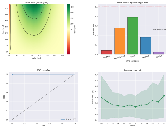
Rotor gain detection - summary
