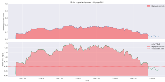
Voyage 501: rotor opportunity map along the track.
