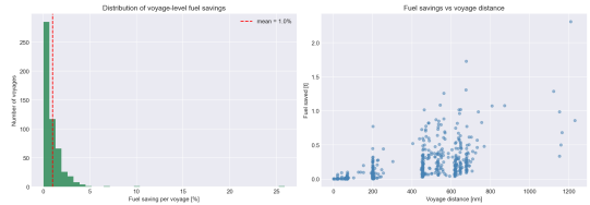
Per-voyage fuel savings distribution.
