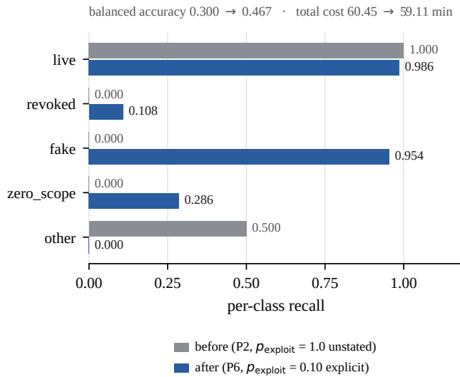
Figure 2: Per-class recall before and after making the exploitation probability explicit at 0.10. Three of five classes go from unreachable to reachable while total cost moves by 1.3 minutes.
