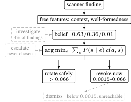
Figure 1: The agent. Two free features produce a belief; the cheapest terminal action follows from the cost matrix. Dashed paths are those the policy takes rarely or never: INVESTIGATE fires on 4% of findings, ESCALATE on none, and DISMISS on no belief the agent can reach. That two of five actions go unused is a result, not an omission.
