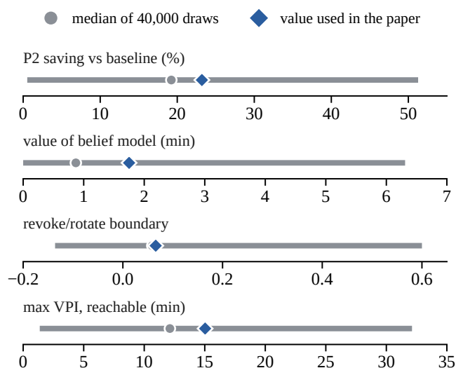
Figure 4: Point estimates against their sampled distributions, 5th to 95th percentile. Every value we quote sits near the median of its distribution, so the cost model is not an outlier among plausible ones—but the intervals are wide enough that quoting any single figure implies a precision the model does not have. A negative boundary means revoke-now never wins in that world.
