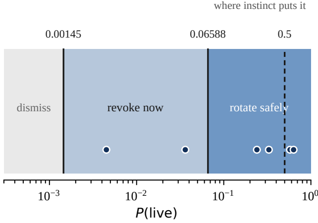
Figure 2: Decision regimes on the reachable line, and the six posteriors the agent can actually hold (dots). The derived boundary between revoking and rotating sits at 0.066; the dashed line at 0.5 is where an engineer sets it by instinct. Everything between the two is dismissed by the naive rule and rotated by ours.
