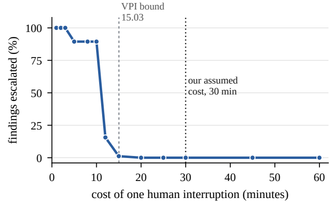
Figure 3: Escalation is a function of one number we guessed. With every other cost fixed at its point estimate, the agent escalates every finding when a human costs three minutes and none when a human costs twenty. Our assumed thirty is well past the crossover; a dedicated triage analyst would not be.
