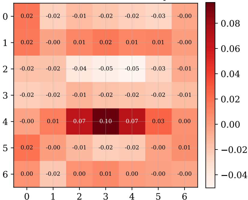
arcface — occlusion sensitivity ( \Delta\text{sim} )
