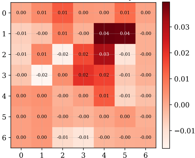
facenet — occlusion sensitivity ( \Delta\text{sim} )
