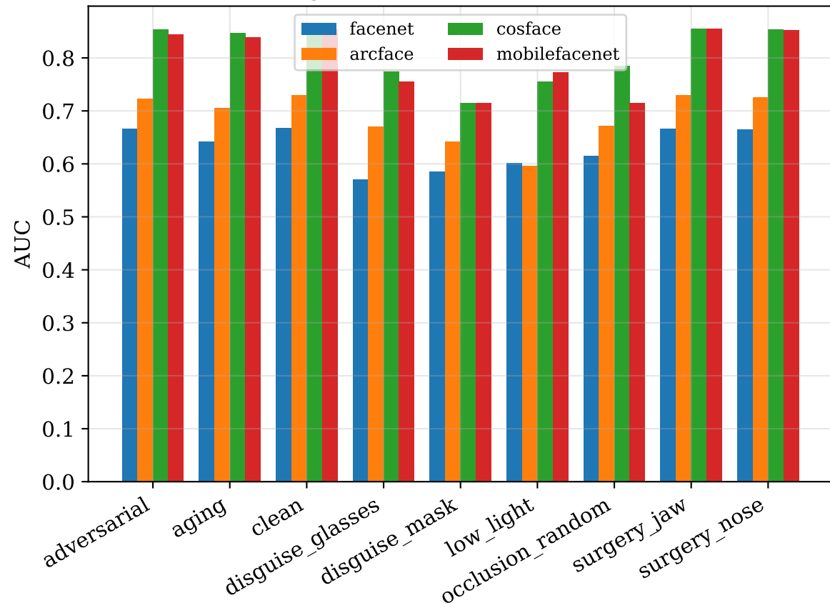
Stage 1: AUC per modification
