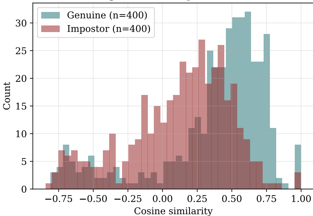
arcface — genuine vs impostor distributions
