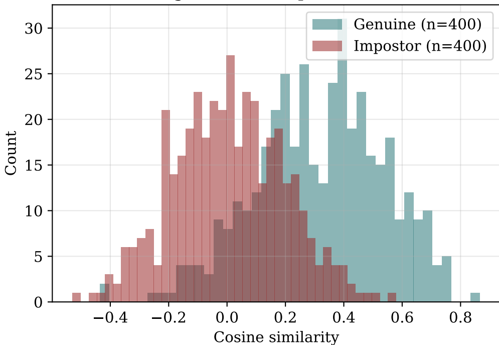
cosface — genuine vs impostor distributions
