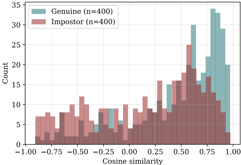
facenet — genuine vs impostor distributions
