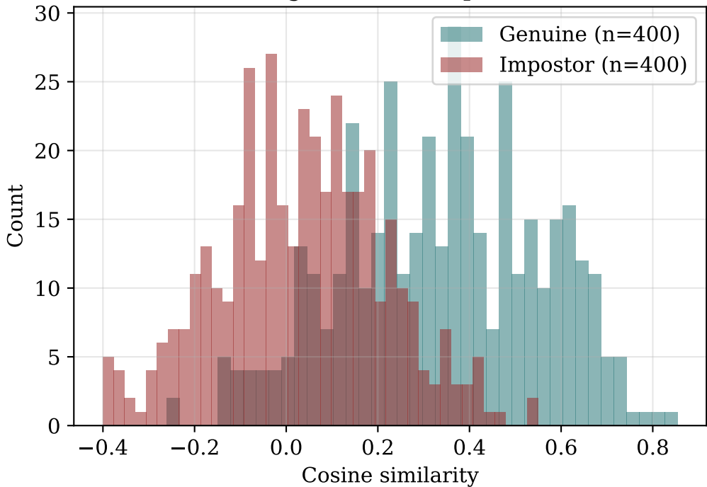
mobilefacenet — genuine vs impostor distributions
